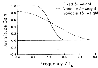
Figure 6. Gain functions for 3-weight digital filters constructed with fixed weights or by the frequency-domain method to yield cutoff frequencies of approximately 0.2f_s . f_s is the sampling rate. The gain function for a 15-weight filter constructed by the frequency-domain method is also shown. Note that unlike the fixed-weight method, the present method allows the 3-weight filters to be improved by adding more weights without altering the cutoff frequency.
